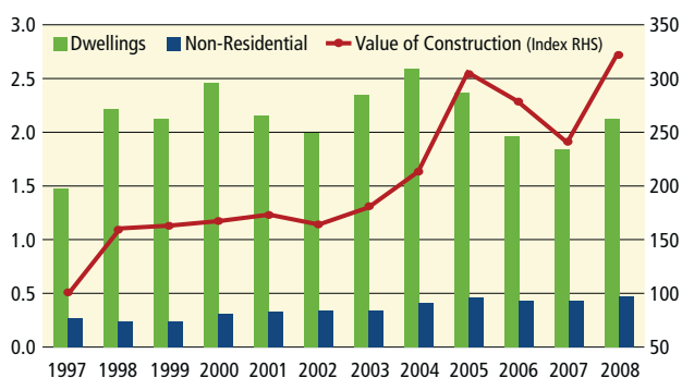
Figure 99: Building activity (000) and construction value, Wellington region. Year ended March. Index: 1997 = 100. Source: Statistics New Zealand
