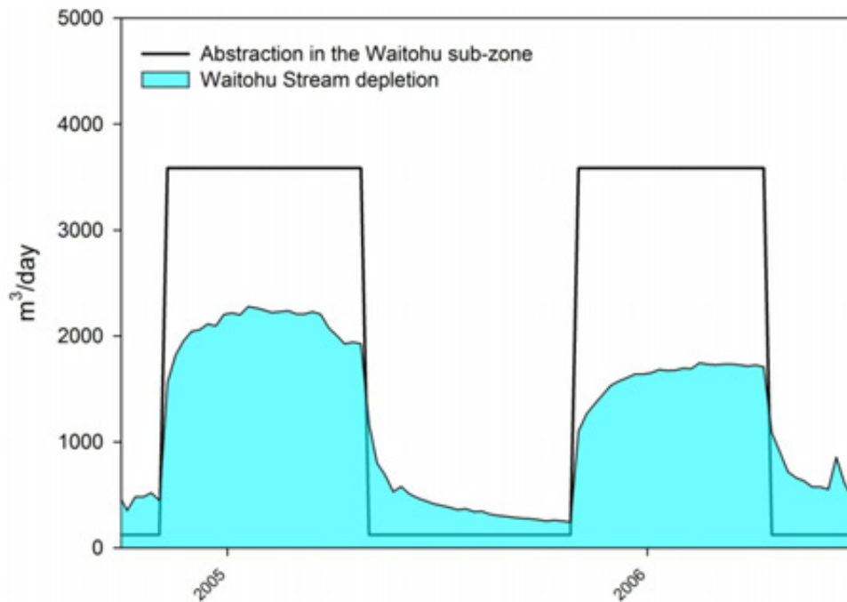
Figure A10: Details of Figure A9-Simulated historic abstraction and associated surface water depletion in the Waitohu sub-zone zone between 2004 and 2006. The plot demonstrates the lag between start and termination of seasonal pumping and surface water depletion. Surface water depletion responds almost immediately to pumping. Abstraction and depletion peak during the summer. The peak depletion rate is approximately 50% of abstraction ( q/Q=0.5 ) and depletion continues through the winter due to rainfall effects.
