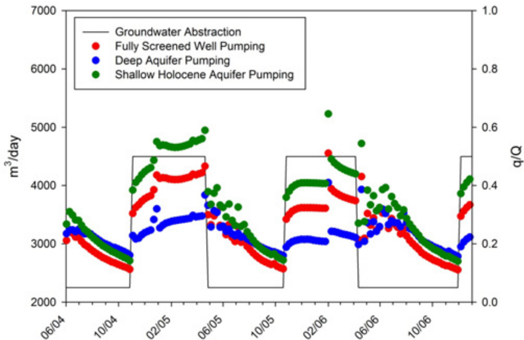
Figure D16: Scenario 4 – surface water depletion resulting from groundwater abstraction from the shallow Holocene sands, deep aquifer and from fully screened wells in the Raumati zone, May 2004 to October 2006
