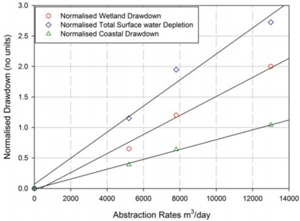
Figure D20: A plot of normalised drawdown/depletion to maximum permissible total surface water depletion, wetland drawdown and coastal drawdown effects against incremental daily abstraction rates
