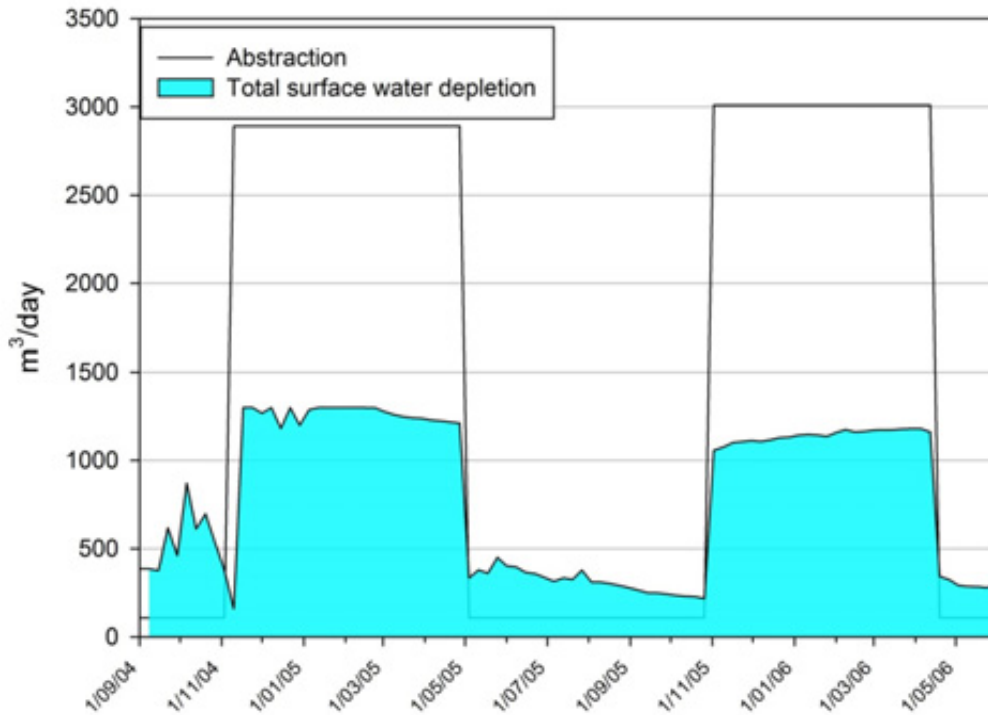
Figure B5: Details of Figure B3 – Simulated historic abstraction and associated surface water depletion in the Te Horo zone between 2004 and 2006. The plot demonstrates the lag between start and termination of seasonal pumping and surface water depletion. Surface water depletion responds almost immediately to pumping. There is a small residual depletion recession throughout the winter which is largely controlled by seasonal rainfall recharge.
