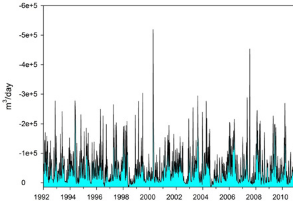
Figure A5: Simulated net natural surface water fluxes to the Waitohu Stream in the Otaki zone when no groundwater abstraction is occurring. The negative fluxes represent flow from groundwater to the stream (i.e. gaining system). This plot shows the net gain over the entire reach of the Waitohu Stream. The plot also shows some positive values during the dry season i.e. net loss from the Waitohu Stream to groundwater.
