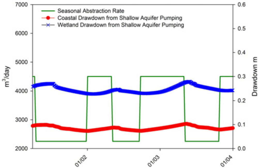
Figure D18: Scenario 4 outputs – simulated wetland and coastal drawdowns when abstraction is from shallow Holocene sands only after pumping at 2,250 m³/day (winter) and 4,500 m³/day (summer)
