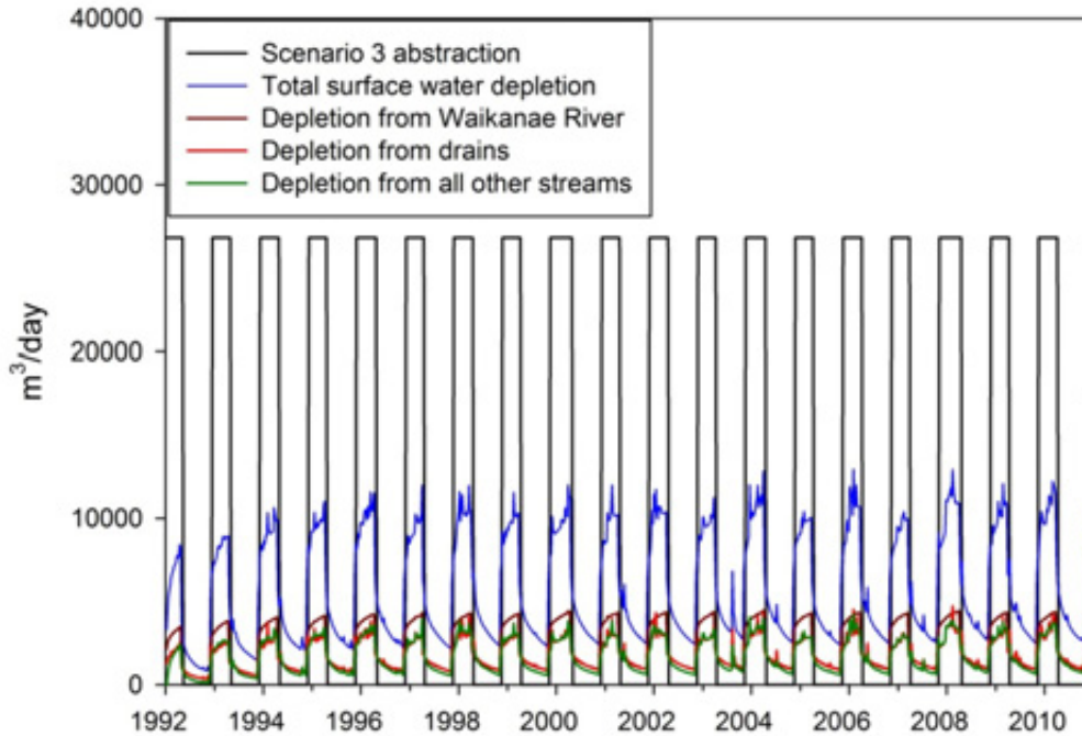
Figure C11: Scenario 3 output – surface water depletion when pumping from Q6 (layers 6 and 7) only of the of the Waikanae zone. Pumping from current consented bores located in the Q4 (50 to 60m deep) at an abstraction rate of 26,826 m 3 /d.
