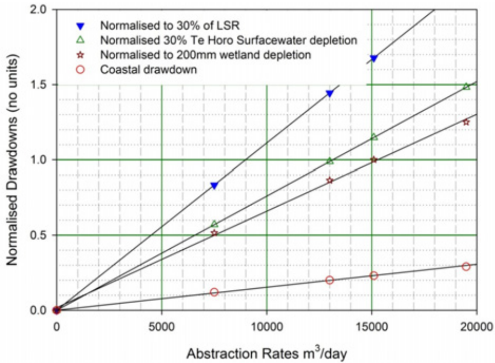
Figure B10: Allocation envelopes abstracting from all three aquifers in the Te Horo zone. Lower Quartile surface recharge is normalised to 30% LQSR, Wetland drawdown is normalised to 0.20m, stream depletion is normalised to 30% of MALF for the zone (60.9 L/s) and drawdown at the coast is normalised to 1m. The normalisation values are the maximum allowable depletions or drawdown to limit adverse environmental effects. A normalised LQSR of 1.0 intersects the abstraction rate at 9,000 m 3 /day (i.e. the maximum abstraction rate equivalent to 30% LQSR). The normalised stream depletion ratio at this abstraction rate is 0.7 or 70% of 60.9 L/s or 3,600 m 3 /day. The coastal drawdown is approximately 0.3m. The normalised wetland drawdown at this abstraction rate is 0.6 (i.e. equivalent to 120mm drawdown).
