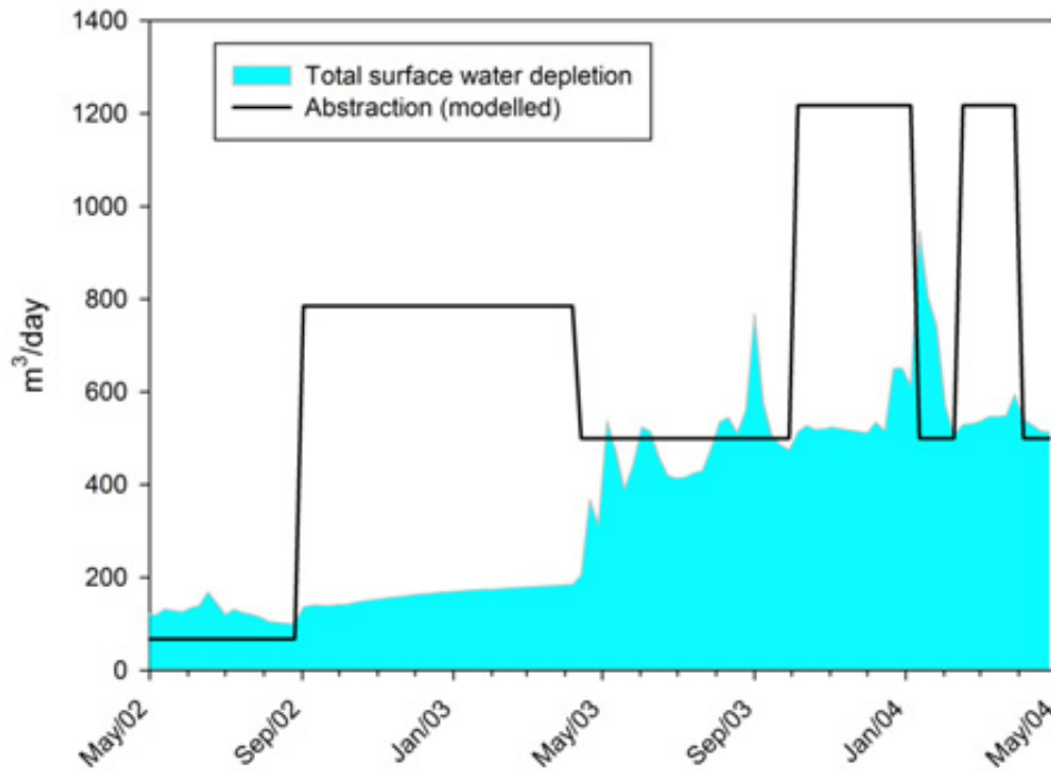
Figure D5: Simulated surface water depletion resulting from groundwater abstraction in the Raumati zone between May 2002 and May 2004
