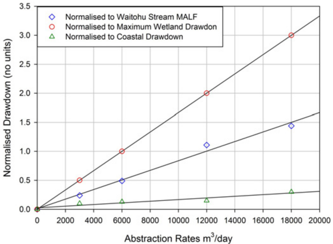
Figure A16: Allocation envelopes abstracting from all three aquifers in the Waitohu sub-zone. Wetland drawdown is normalised to 0.2m, stream depletion is normalised to 30% of MALF (45L/s) and drawdown at the coast is normalised to 1m. The normalisation values are the maximum allowable depletions or drawdown to limit adverse environmental effects. A normalised wetland drawdown of 1.0 intersects the abstraction rate at 6,000m³/day (i.e. the proposed maximum abstraction rate to limit wetland drawdown to less than 200mm (0.20m)).
