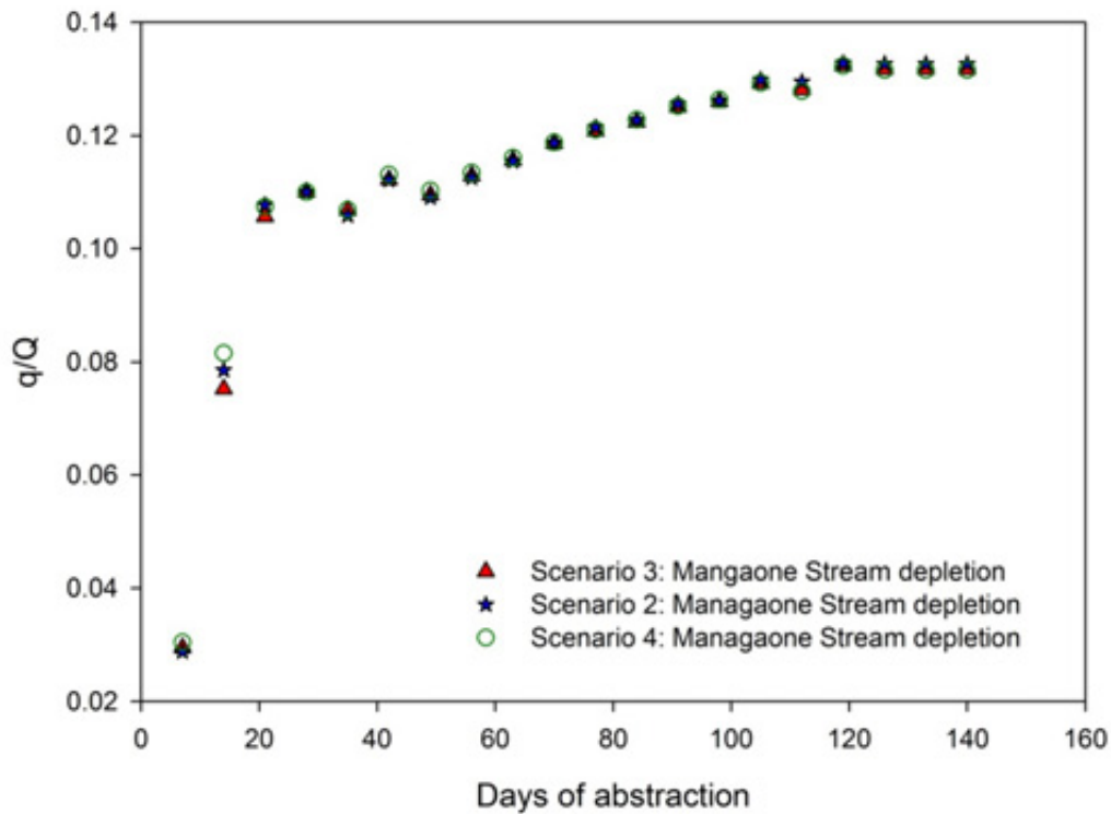
Figure B8: Scenarios 2 to 4 – ratio of surface water depletion ( q ) to pumping rate ( Q ) for the Mangaone Stream – abstracting from all the aquifers at 7,500 m 3 /day (Scenario 2), 15,000 m 3 /day (Scenario 3) and 20,000 m 3 /day (Scenario 4)
