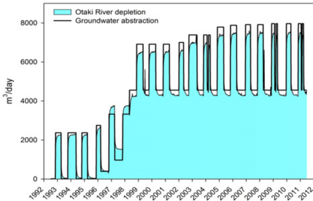
Figure A6: Simulated historic abstraction and associated surface water depletion in the Otaki zone (1992-2012). A depletion equivalent to 85 to 95% of the abstraction rate occurs within the timeframe of seasonal abstraction and recedes over the winter months.
