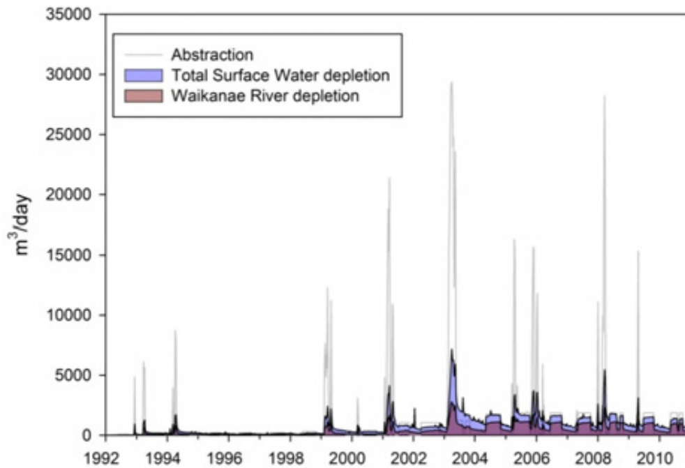
Figure C4: Simulated total surface water depletion resulting from abstraction in the Waikanae zone from all consented bores between 1992 and 2012. The relatively low surface water depletion when compared to groundwater abstraction was due to the short period of high abstractions.
