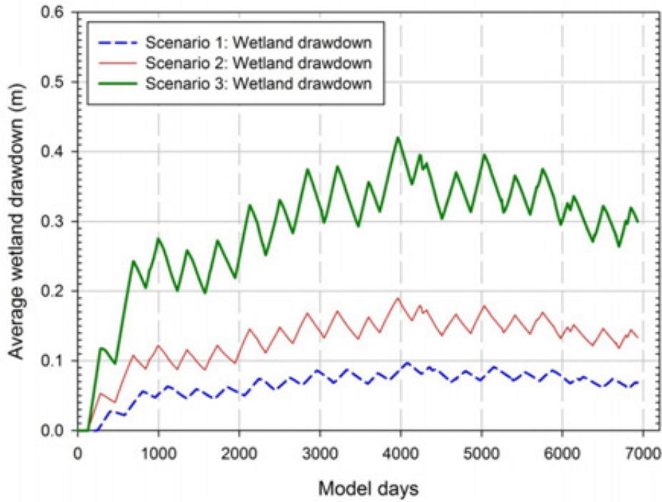
Figure A14: Scenarios 1 to 3 output – wetland drawdowns in the Waitohu zone resulting from pumping an array of synthetic fully screened wells outside Q1 gravels at 3,000m 3 /day (Scenario 1), 6,000m 3 /day (Scenario 2) and 12,000m 3 /day (Scenario 3) for a 19 year model run
