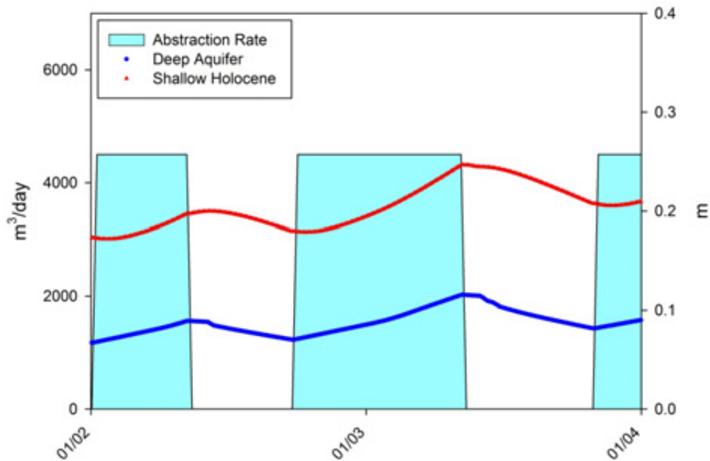
Figure D12: Simulated drawdown associated with seasonal abstraction at 4,500 m 3 /day from the shallow Holocene aquifer and deep aquifer respectively over the 2002/03 period
