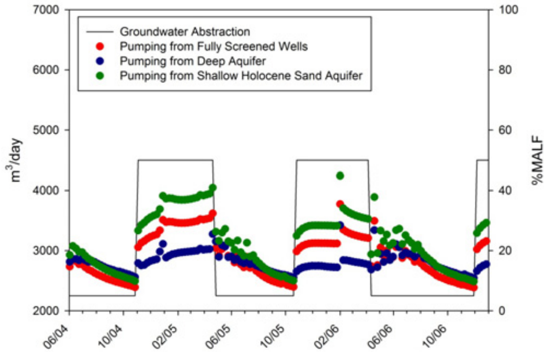
Figure D17: Scenario 4 – surface water depletion (%MALF) resulting from groundwater abstraction from the shallow Holocene sands, deep aquifer and from fully screened wells in the Raumati zone (2004-2006)
