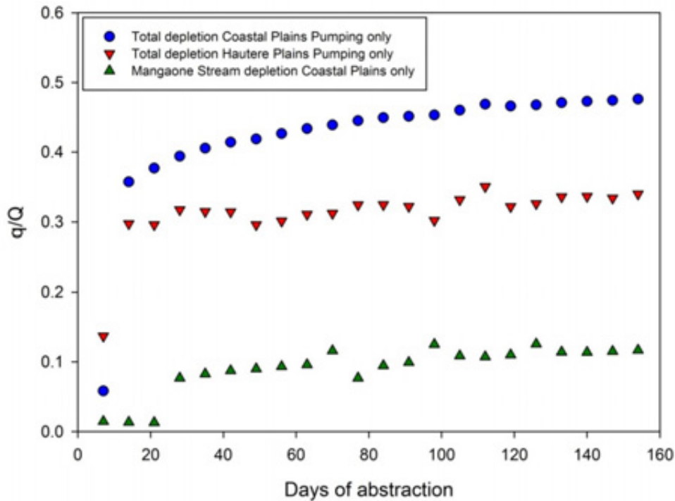
Figure B6: Scenario 1 – ratio of surface water depletion ( q ) to pumping rate ( Q ) when abstracting from deep aquifers of the Coastal and Hautere plains in the Te Horo Zone. The figure shows a fast response in stream depletion to abstraction from deep aquifers >60m for both the Hautere and Coastal zones.
