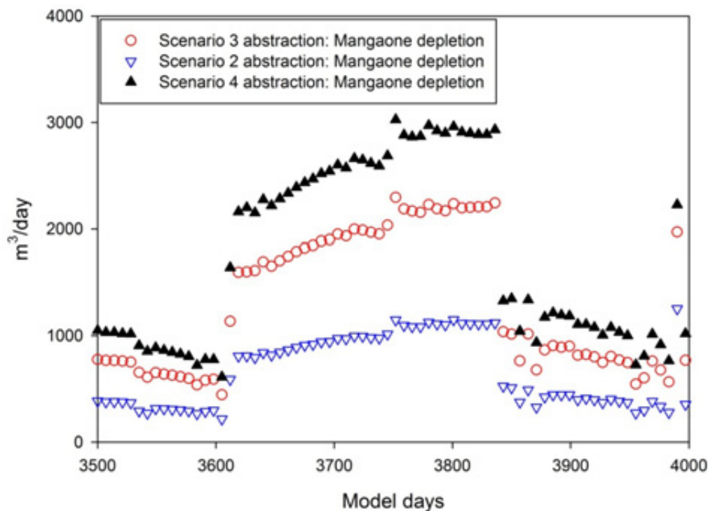
Figure B7: Scenarios 2 to 4 surface water depletion in the Mangaone Stream resulting from pumping an array of synthetic bores located in the three identified aquifers of the Te Horo zone. Abstraction from the aquifer at 7,500m 3 /day (Scenario 2), 15,000m 3 /day (Scenario 3) and 20,000m 3 /day (Scenario 4) extracted from model days 3500 to 4000 from 19 years (6930 days) simulation.
