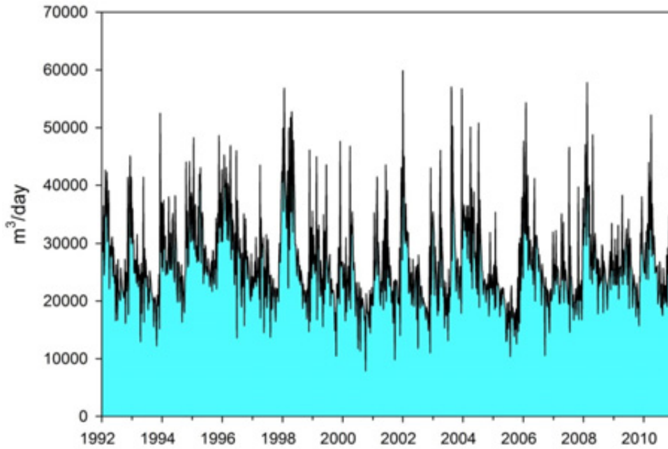
Figure A4: Simulated net natural surface water fluxes to the Otaki River in the Otaki groundwater management zone when no groundwater abstraction is occurring. The positive fluxes represent flow from the Otaki River to groundwater (i.e. losing system). This plot shows the net loss over the entire reach of the Otaki River.
