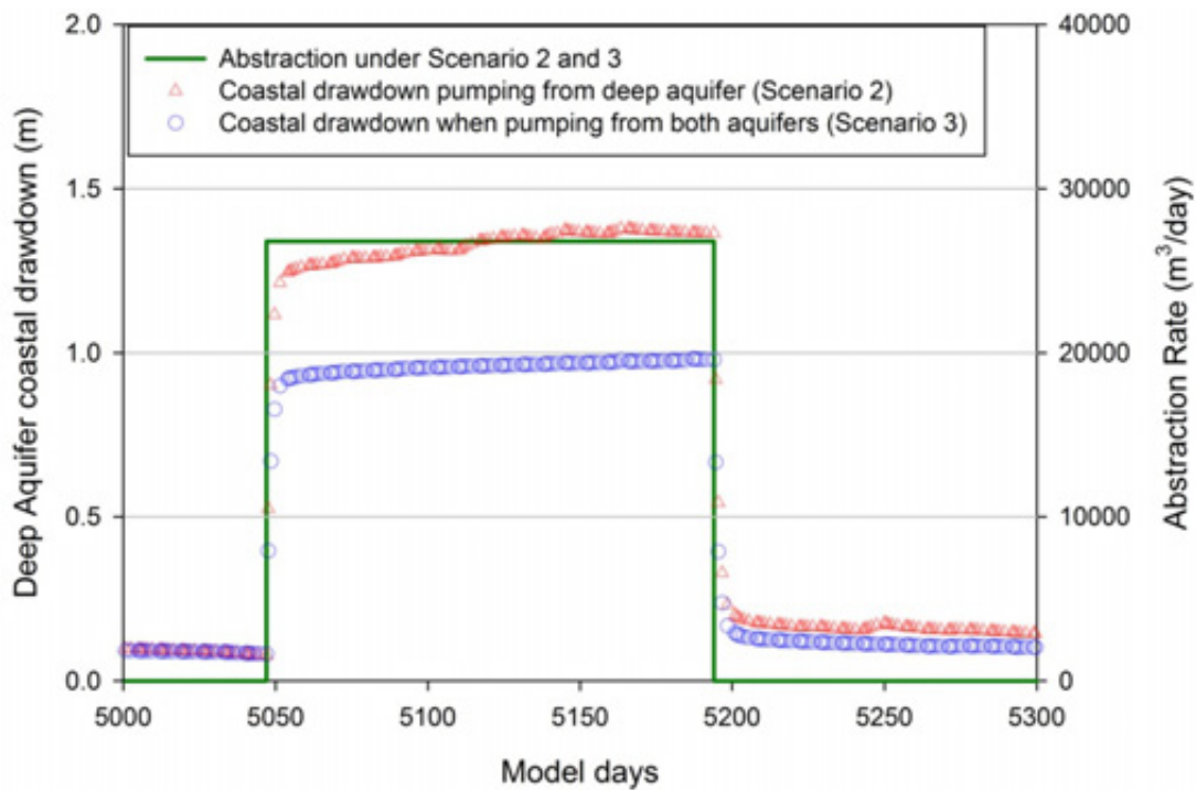
Figure C14: Scenarios 2 and 3 – coastal drawdown to pumping rate (Q) for scenarios 2 and 3 pumping. Abstractions from the deep Q6 aquifer > 60m bgl (Scenario 2) and Q4 (Scenario 3).
