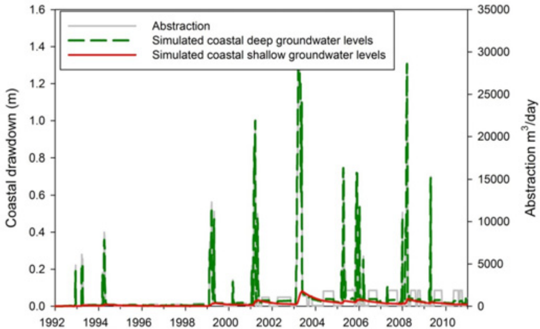
Figure C7: Simulated coastal drawdown resulting from abstraction in the Waikanae zone from all consented bores between 1992 and 2012. The quick response in coastal drawdown and complete recovery in deep groundwater levels indicates that although the potential for saltwater intrusion is high, deep coastal aquifers have quick recovery to re-establish the seaward discharge of groundwater. The shallow coastal groundwater behaviour is similar to wetland responses and do not recover completely from high groundwater abstractions.
