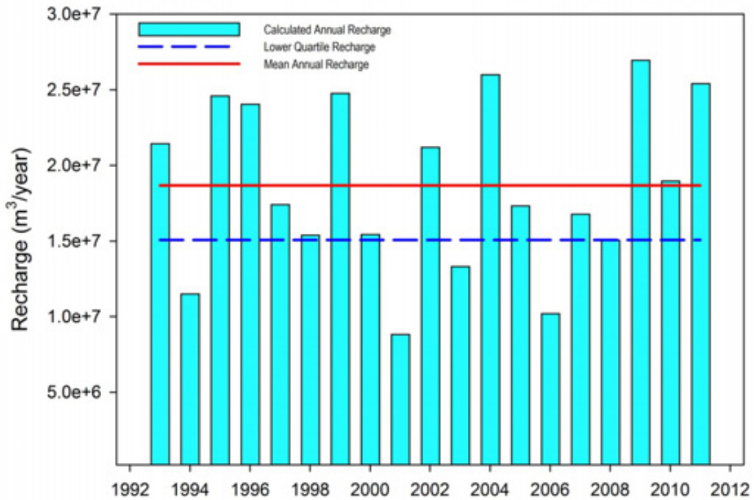
Figure B2: Modelled annual rainfall recharge (1993-2011) for the Te Horo zone between 1992 and 2012. A mean recharge 51,161 m 3 /day is indicated as is the lower quartile value of 41,301 m 3 /day (dashed line).
