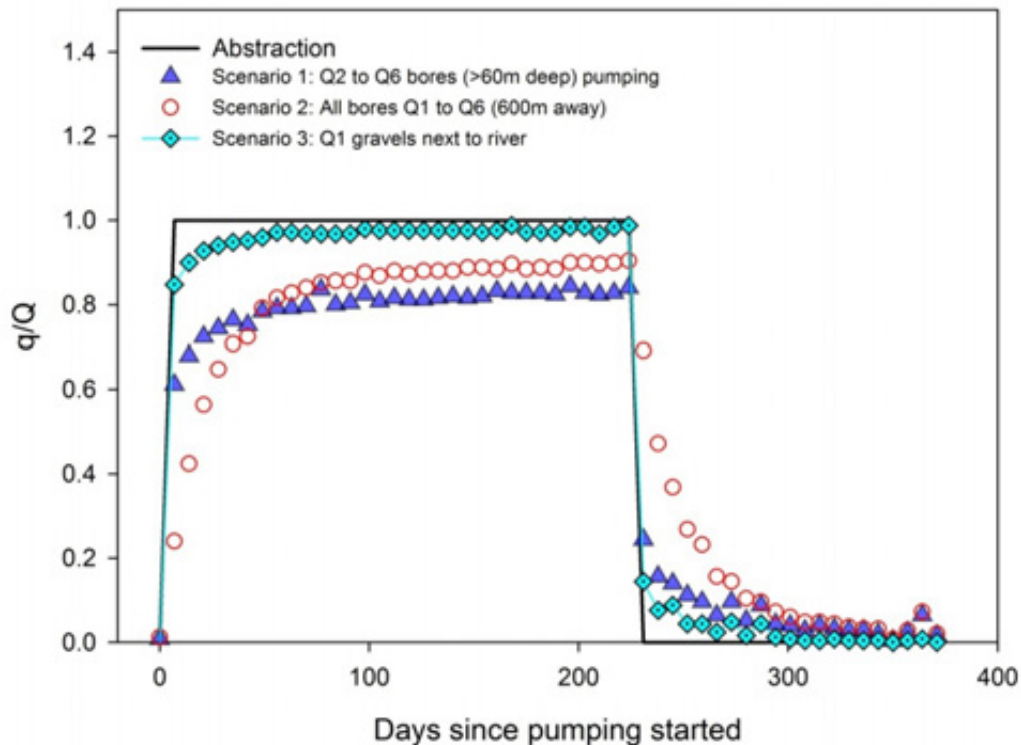
Figure A8 shows simulated surface water depletion resulting from synthetic abstractions in the Otaki River sub-zone. The model predicts that total seasonal abstraction depletion is between 80 and 100% of the total abstraction rate thereby indicating a high degree of connectivity between the aquifer and the Otaki River.
