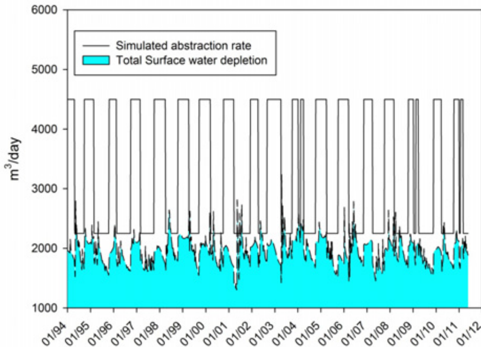
Figure D13: Scenario 4 results – simulated cumulative stream depletion resulting from continuous abstraction (4,500 m 3 /day summer, 2,250 m 3 /day winter) over the 1994 to 2012 period
