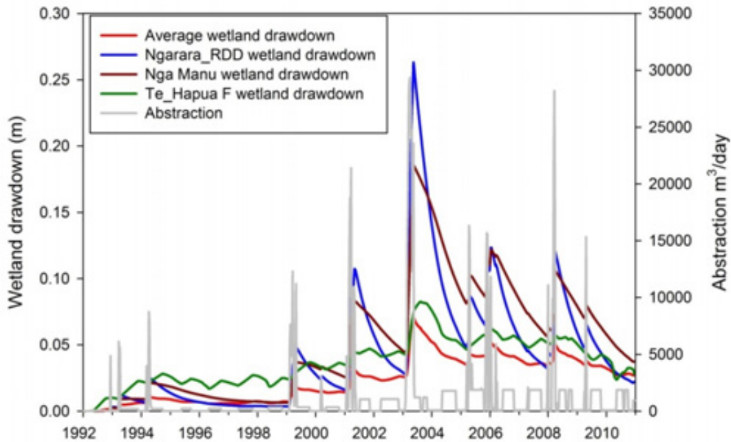
Figure C5: Simulated wetland drawdown resulting from abstraction in the Waikanae zone from all consented bores between 1992 and 2012. The quick response in wetland drawdown and un-complete recovery in wetland levels indicates that a continued increase in abstraction may not be sustainable in this zone.
