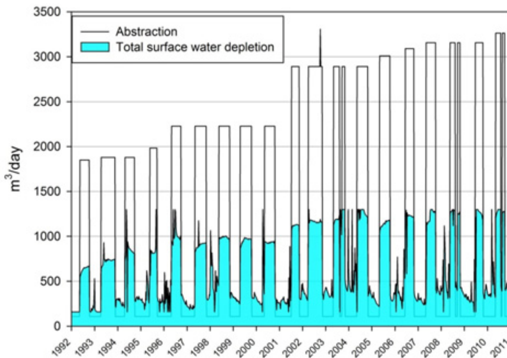
Figure B4: Simulated historic abstraction and associated surface water depletion in the Te Horo zone (1992-2012). A depletion equivalent to 35 to 40% of the abstraction rate occurs within the timeframe of seasonal abstraction and recedes over the winter months.
