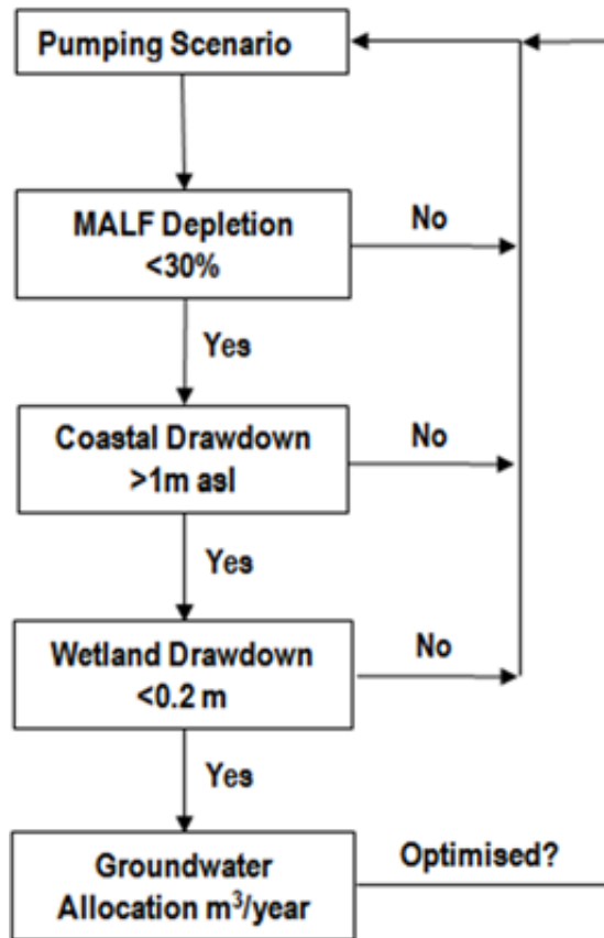
Figure 6: Schematic illustration of the iterative modelling process utilised evaluate pumping scenarios and determine groundwater allocation limits
