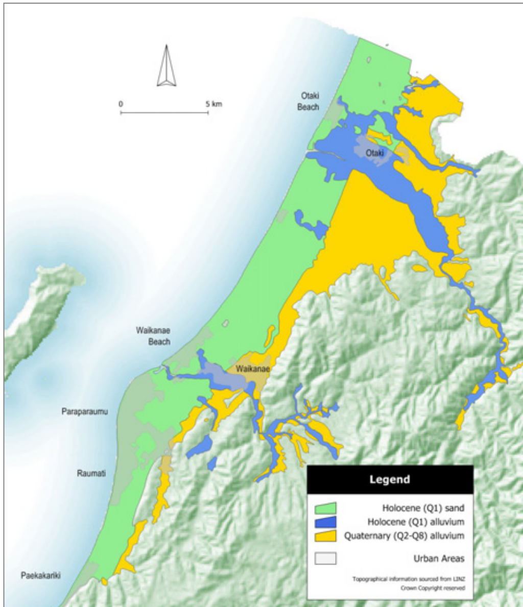
Figure 1: Simplified geological map of the Kapiti Coast (adapted from GNS Wellington QMap coverage). The figure shows the spatial distribution of the Q1 sand deposits (green) along the coastal margin, the Q1 alluvium along the margins of the Otaki River, Waikanae River and Waitohu Stream (blue) as well as the older Quaternary sand and gravel sediments (yellow) which form a succession of alluvial terraces along the western margin of the Tararua foothills and extend westwards toward the coastal underneath the younger Q1 sand and gravel materials.
