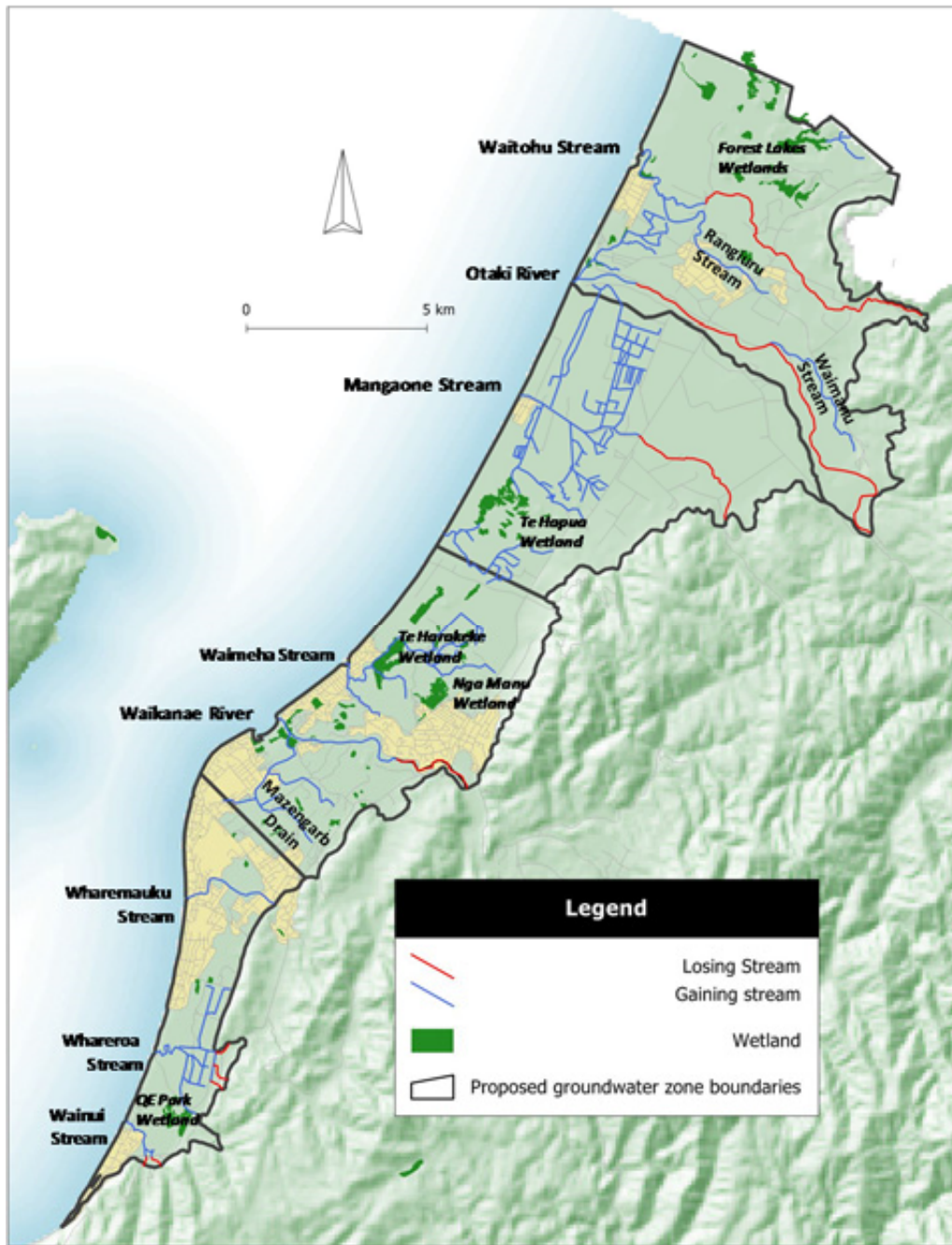
Figure 2: Spatial distribution of gaining and losing streams and major wetlands on the Kapiti Coast
