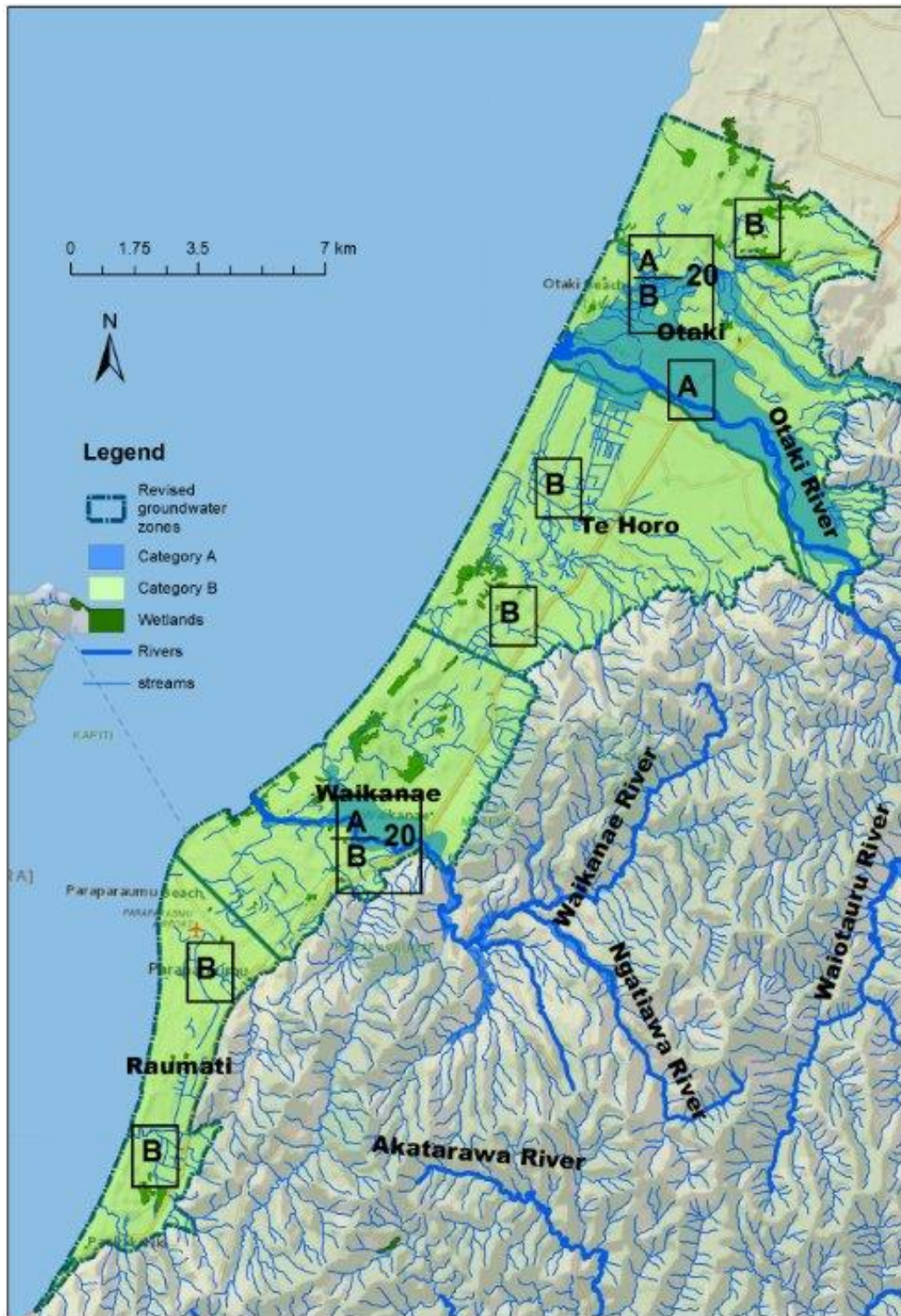
Figure 3: Spatial and depth distribution of proposed hydraulic connectivity zones for the Kapiti Coast
