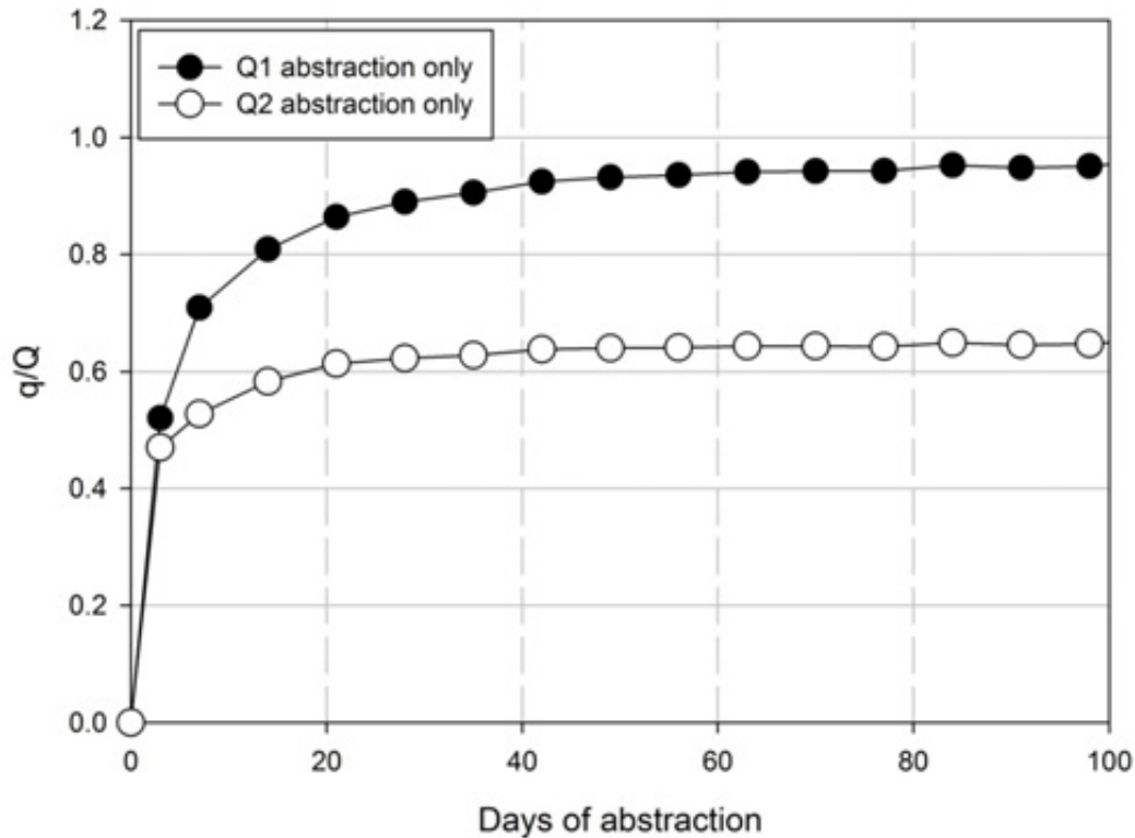
Figure C9: Scenario 1 – ratio of surface water depletion ( q ) to pumping rate ( Q ) from pumping an array of synthetic bores located in the shallow unconfined and semi-confined aquifers in Q1 (ground surface to about 20 m depth) and Q2 (between 20 m to 30 m depth) gravels
