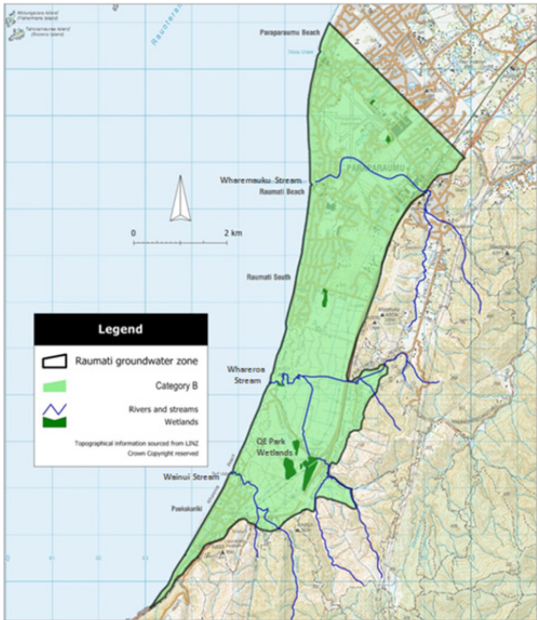
Figure 10: Map of the proposed hydraulic connectivity zonation for the Raumati groundwater zone showing the location of significant surface water features
