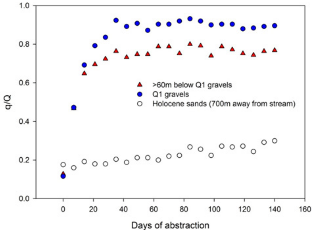
Figure A11: Ratio of surface water depletion ( q ) to pumping rate ( Q ) for the Waitohu sub zone pumping from Q1 gravels (only), Q2 to Q6 below Q1 gravels (only) and Holocene sands 700m from the Waitohu Stream
