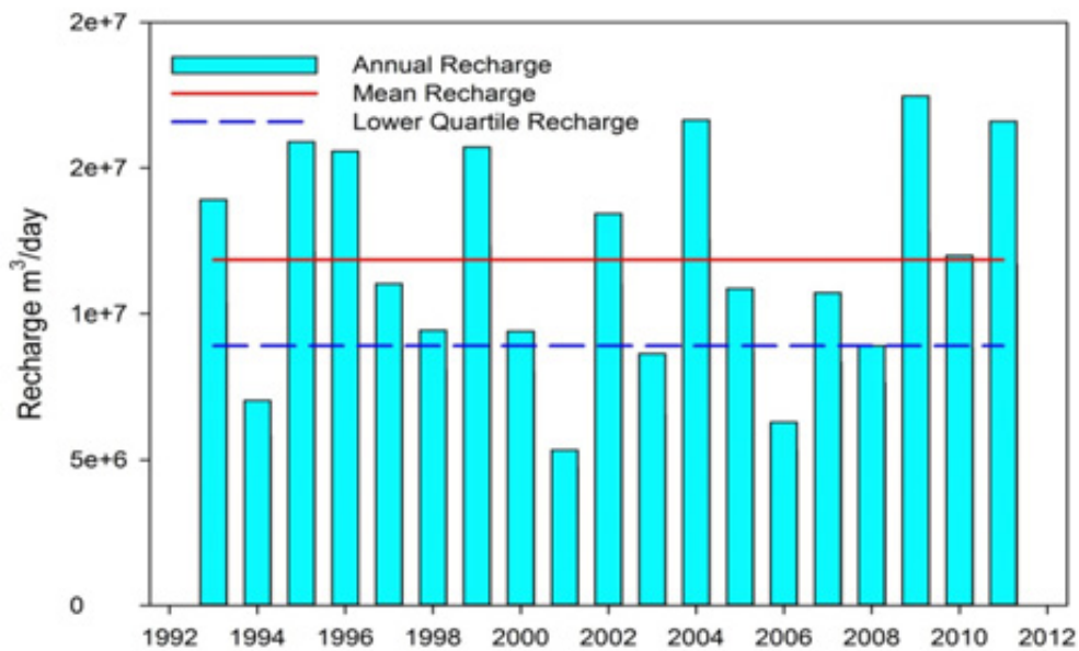
Figure A3: Modelled annual rainfall recharge (1993-2011) for the Waitohu sub-zone between 1992 and 2012. A mean annual recharge of 11.8 \times 10^6 \text{m}^3 is indicated as is the lower quartile value of 8.9 \times 10^6 \text{m}^3 (dashed line).
