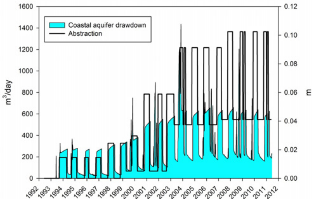
Figure D7: Simulated historic abstraction and associated coastal aquifer groundwater level drawdown. A maximum average coastal drawdown of 0.06 m occurs within the timeframe of seasonal abstraction. Abstraction for municipal supply also occurs over the winter months (2004-2011) and coastal aquifer groundwater levels do not recover completely from cumulative abstractions.
