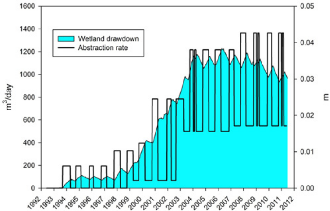
Figure D6: Simulated historic abstraction and associated shallow (Holocene sands) groundwater level drawdown in the vicinity of wetlands in the Raumati zone (1992-2011). A maximum average wetland drawdown of 0.038 m occurs within the timeframe of seasonal abstraction. Abstractions for municipal supply also occur over the winter months (2004-2011) and wetland shallow groundwater levels do not recover completely from cumulative abstractions.
