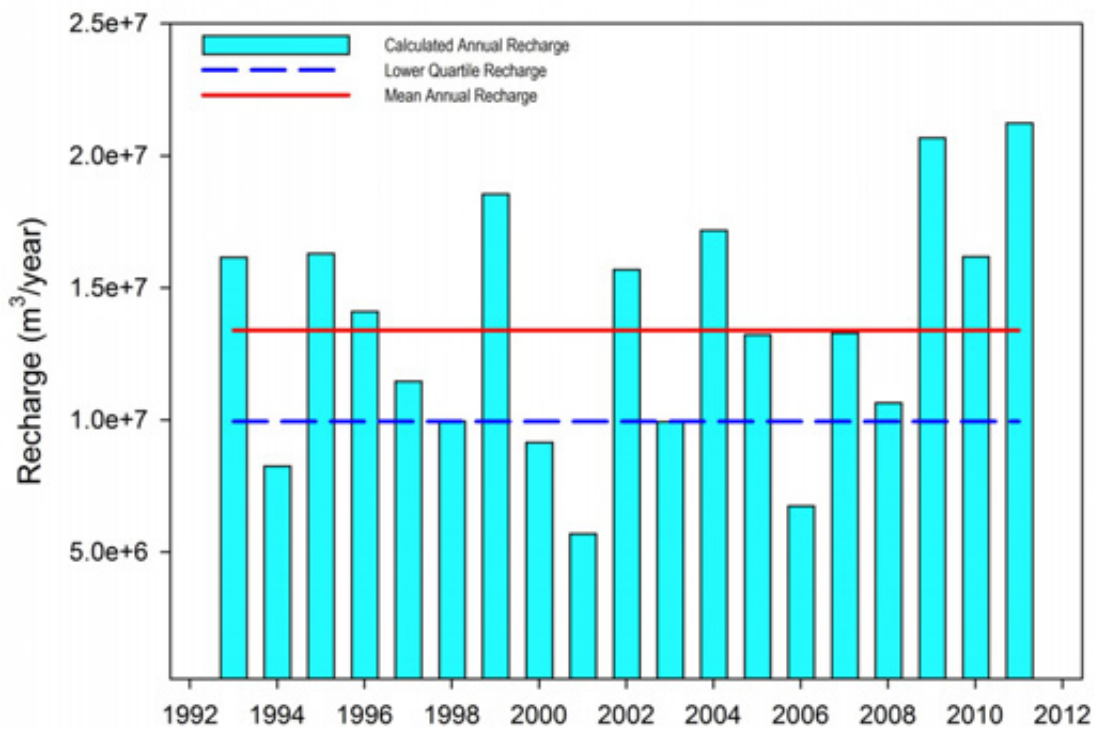
Figure C2: Modelled annual rainfall recharge (1993-2011) for the Waikanae zone between 1992 and 2012. A mean recharge 13.4 \times 10^6 m 3 /year is indicated as is the lower quartile value of 9.94 \times 10^6 m 3 /year (dashed line).
