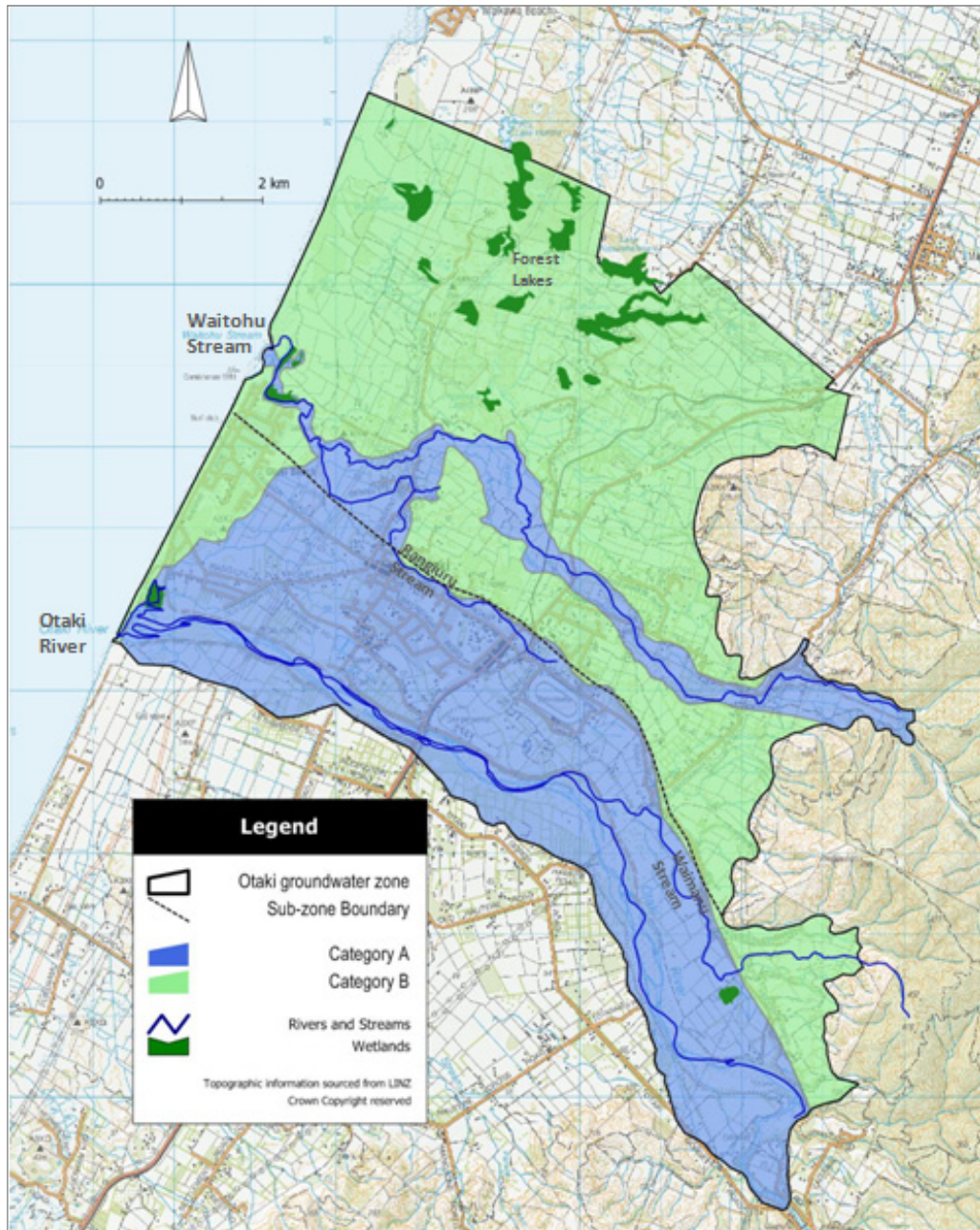
Figure 7: Map of the proposed hydraulic connectivity zonation for the Otaki groundwater zone showing the location of significant surface water features and denoting the extent of the Otaki River and Waitohu sub-zones
