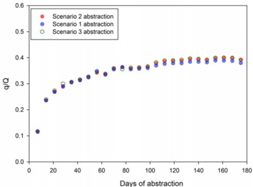
Figure A13: Scenarios 1 to 3 – ratio of surface water depletion (q) to pumping rate (Q) in the Waitohu zone resulting from pumping an array of synthetic fully screened wells outside Q1 gravels at 3,000m³/day (Scenario 1), 6,000m³/day (Scenario 2) and 12,000m³/day (Scenario 3) for 180 days seasonal abstraction
