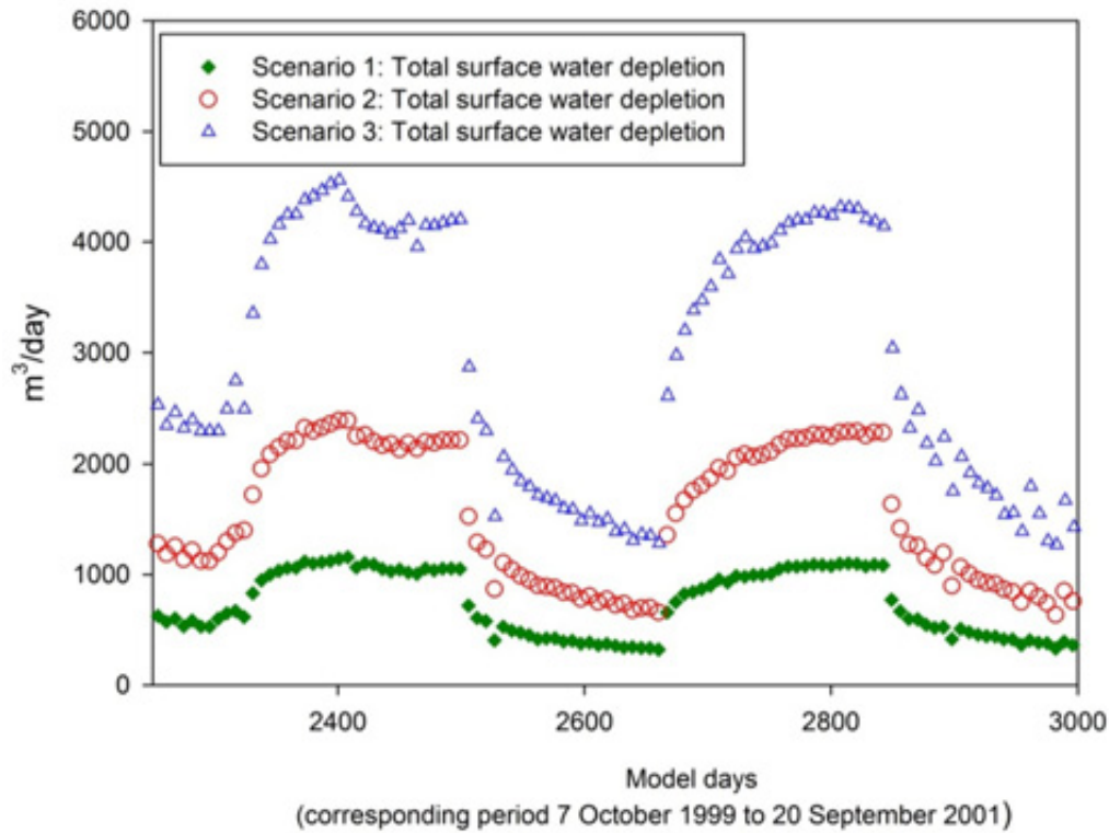
Figure A12: Scenarios 1 to 3 output – surface water depletion in the Waitohu zone resulting from pumping an array of synthetic fully screened wells outside Q1 gravels at 3,000m³/day (Scenario 1), 6,000m³/day (Scenario 2) and 12,000m³/day (Scenario 3) for 180 days seasonal abstraction
