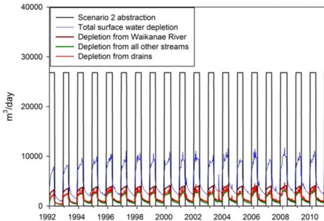
Figure C10: Scenario 2 output – surface water depletion when pumping from Q6 (layers 6 and 7) only of the of the Waikanae zone. Pumping from current consented bores located in the Q6 (> 60m deep) at an abstraction rate of 26,826 m 3 /d.
