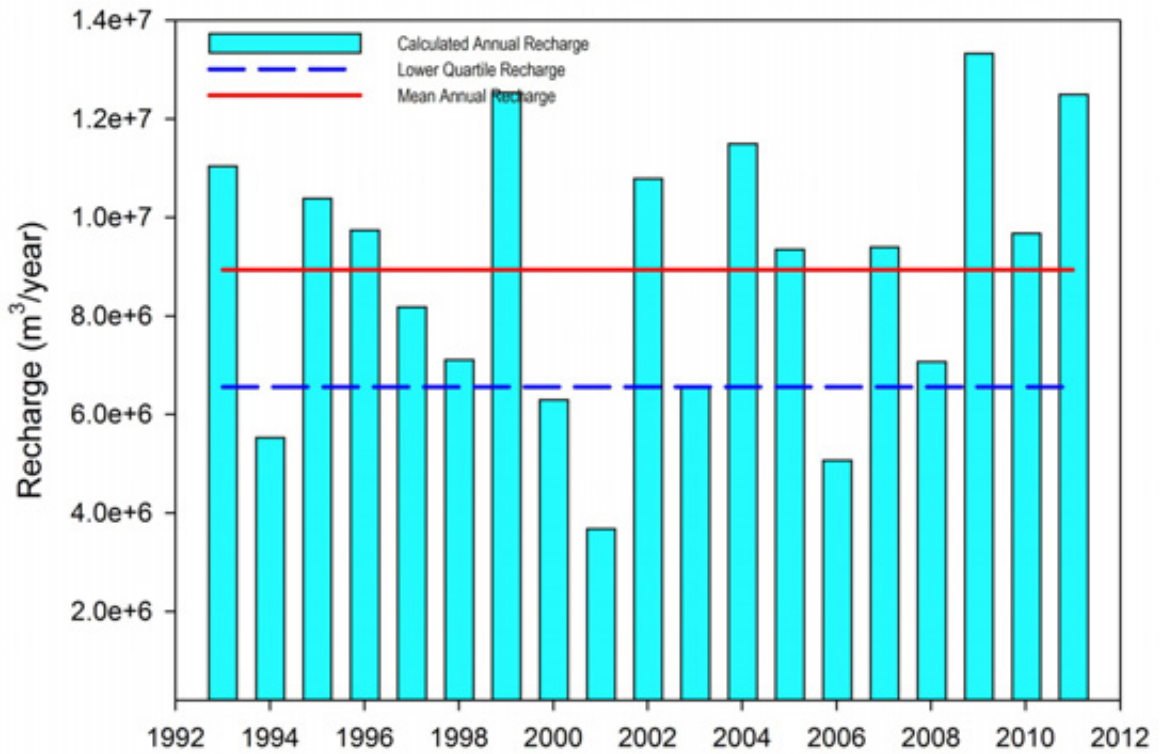
Figure D2: Modelled annual rainfall recharge (1993-2011) for the Raumati zone (mean recharge 8.94 \times 10^6 \text{ m}^3/\text{year} )
