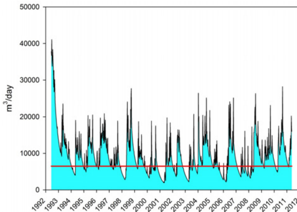
Figure D3: Simulated groundwater discharge to surface water (All streams in the Raumati Catchment) when there is no groundwater abstraction in the Raumati water management zone (1992-2011). Note the modelled summer baseflow is closely related with the 7 day MALF although less than MALF in some years. The extra contribution to MALF comes from drains and upstream discharges.
