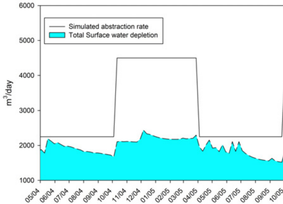
Figure D14: Scenario 4 results – simulated cumulative stream depletion resulting from continuous abstraction (4,500 m 3 /day summer, 2,250 m 3 /day winter) between May 2004 and October 2005
