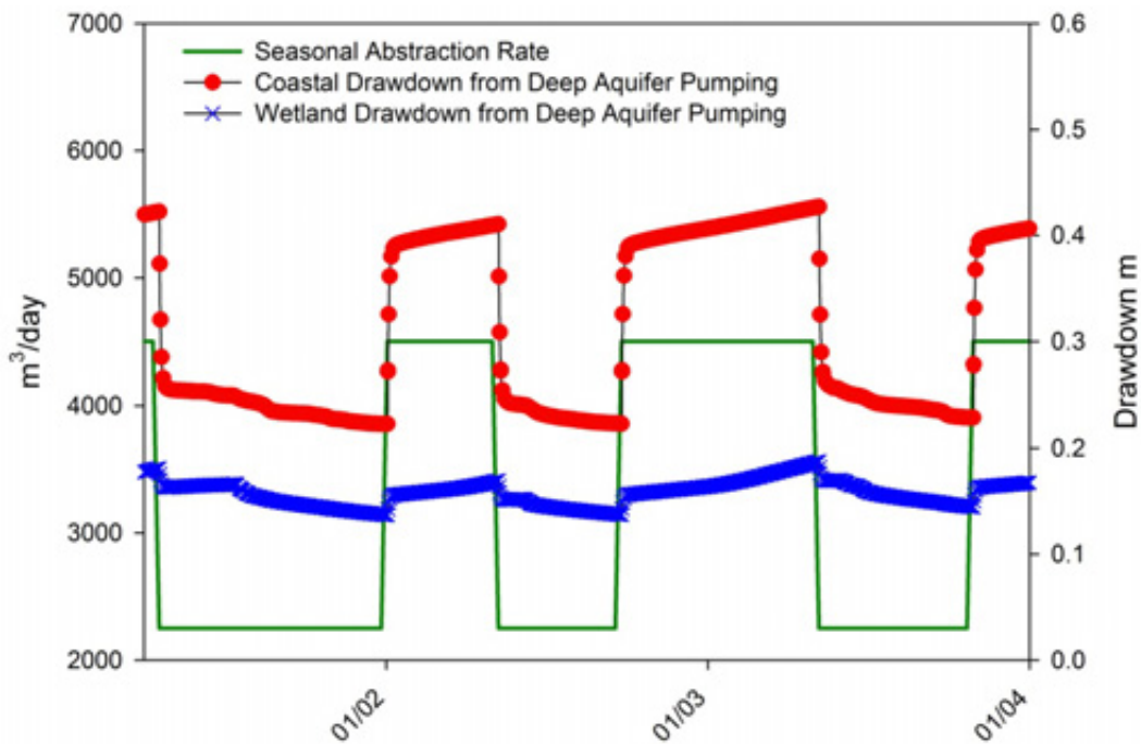
Figure D19: Scenario 4 – simulated wetland and coastal drawdown resulting from abstraction from the deep aquifer at a rate of 2,250 m³/day (winter) and 4,500 m³/day (summer)
