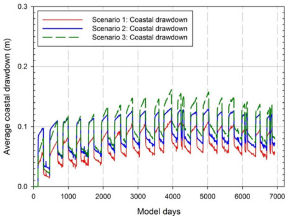
Figure A15: Scenarios 1 to 3 output – coastal aquifer drawdowns in the Waitohu zone resulting from pumping an array of synthetic fully screened wells outside Q1 gravels at 3,000m 3 /day (Scenario 1), 6,000m 3 /day (Scenario 2) and 12,000m 3 /day (Scenario 3) for a 19 year model run
