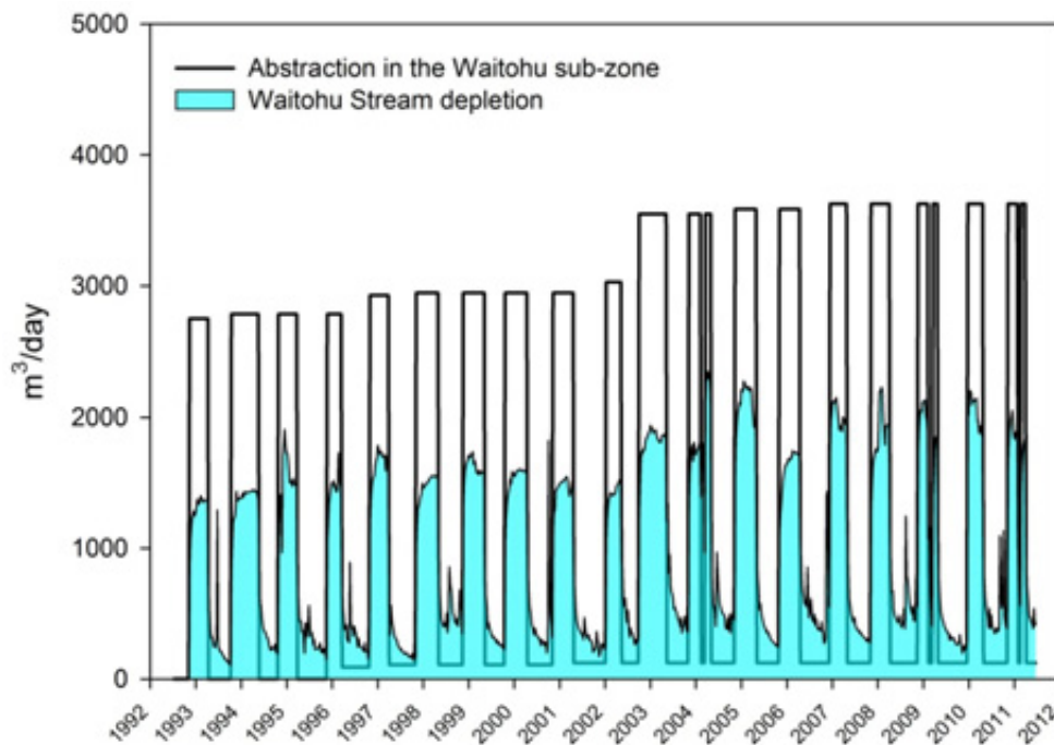
Figure A9: Simulated historic abstraction and associated surface water depletion in the Waitohu sub-zone (1992-2012). A depletion equivalent to 45 to 60% of the abstraction rate occurs within the timeframe of seasonal abstraction and recedes over the winter months.
