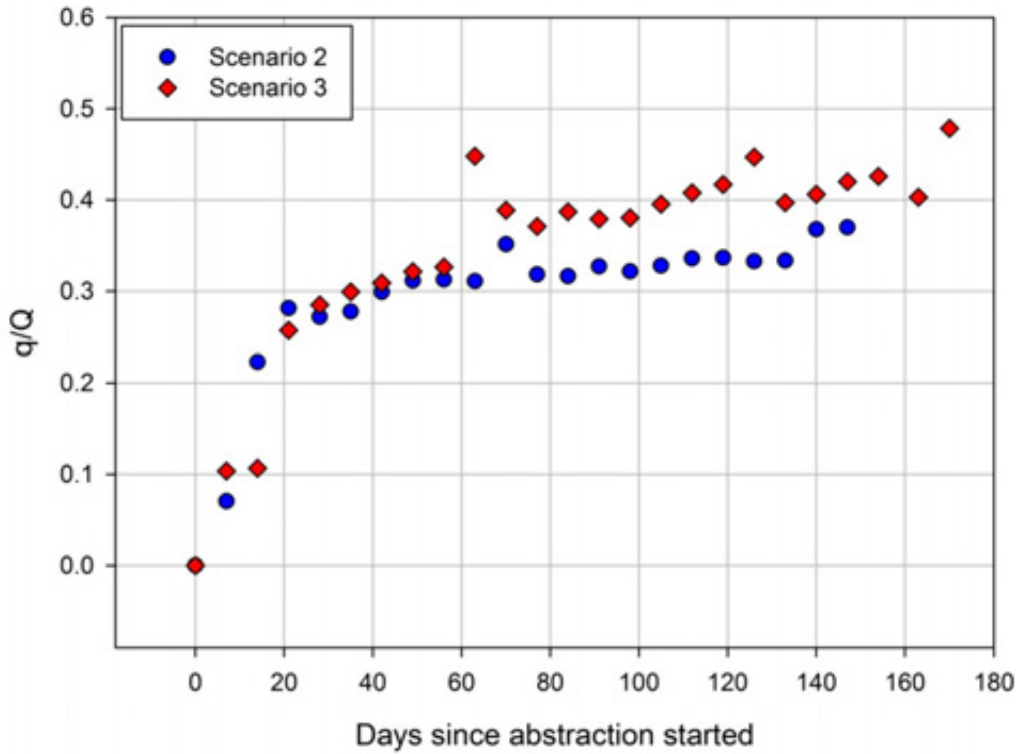
Figure C12: Scenario 2 and 3 – ratio of surface water depletion (q) to pumping rate (Q) for the Waikanae zone
