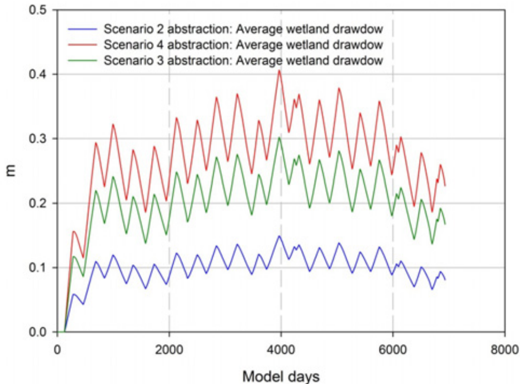
Figure B9: Scenarios 2 to 4 – Wetland drawdown averaged over the six wetlands in the Te Hapua wetland complex. Wetland drawdown when wells are abstracting from all aquifers at 7,500 m 3 /day (Scenario 2), 15,000 m 3 /day (Scenario 3) and 20,000 m 3 /day (Scenario 4).
