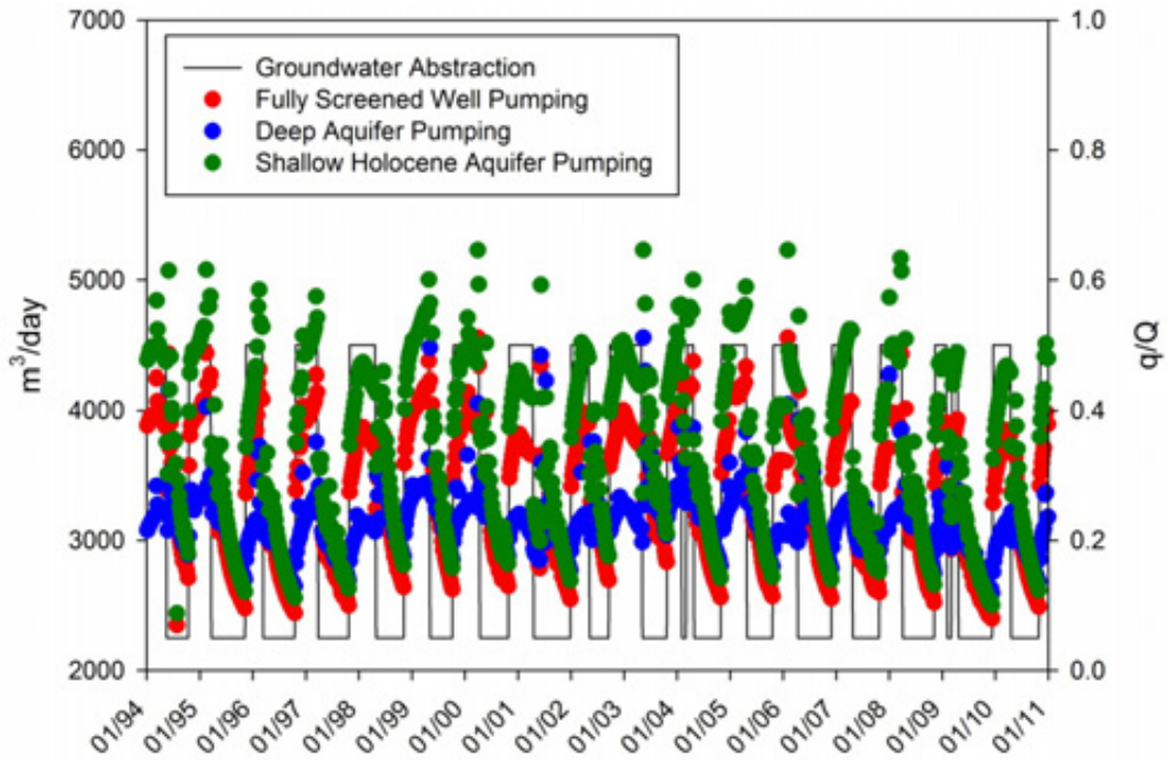
Figure D15: Scenario 4 – surface water depletion resulting from groundwater abstraction from the shallow Holocene sands, deep aquifer and from fully screened wells in the Raumati zone, 1994 to 2012
