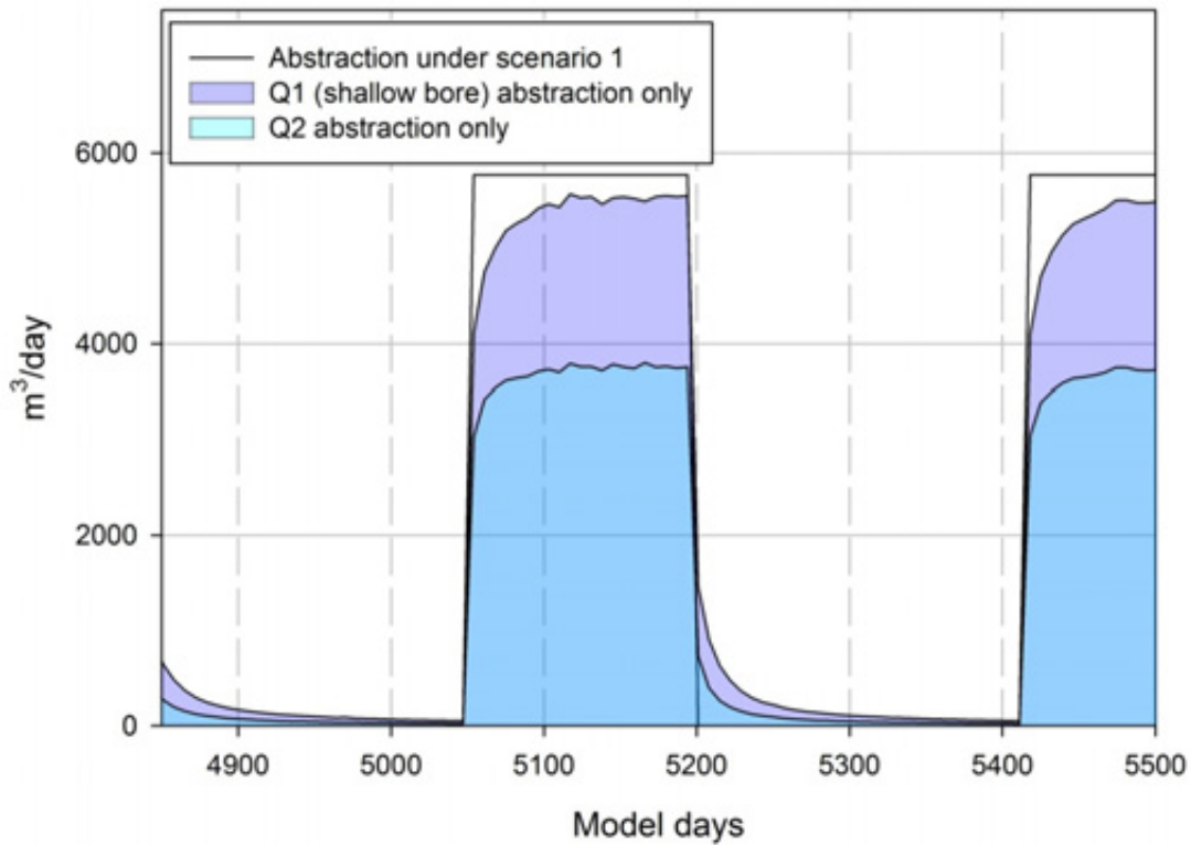
Figure C8: Scenario 1 output – total water depletion in the Waikanae zone from pumping an array of synthetic bores located in the shallow unconfined and semi-confined aquifers in Q1 (ground surface to about 20 m depth) and Q2 (between 20 m to 30 m depth) gravels
