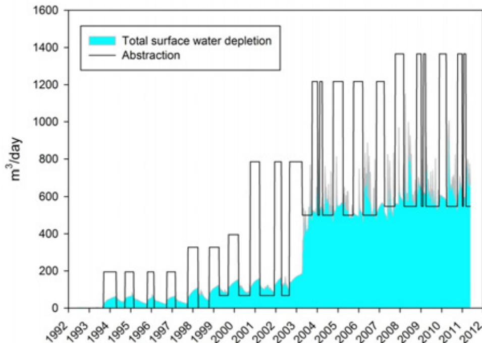
Figure D4: Simulated historic abstraction and associated surface water depletion in the Raumati zone (1992 – 2012). A depletion equivalent to 50 to 70% of the abstraction rate occurs within the timeframe of seasonal abstraction and recedes over the winter months.
