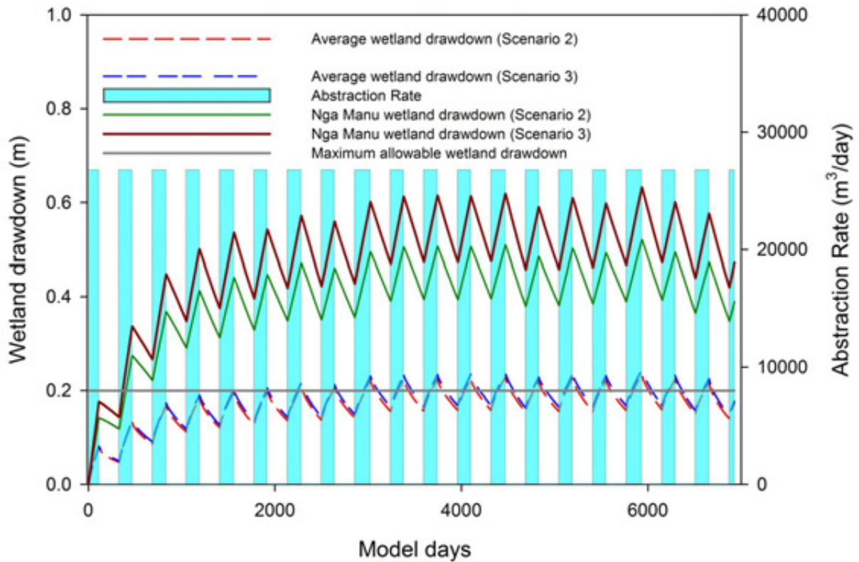
Figure C13: Scenarios 2 and 3 – Simulated wetland drawdown for the Waikanae zone for 19 years of simulation at a seasonal pumping rate of 26,960 m 3 /day for scenarios 2 and 3. Plots show wetland drawdowns (average of 24 wetlands) and drawdown in the nationally significant Nga Manu wetland for the simulation period. The recommended maximum allowable abstraction effect on wetlands is a drawdown of 0.20m.
