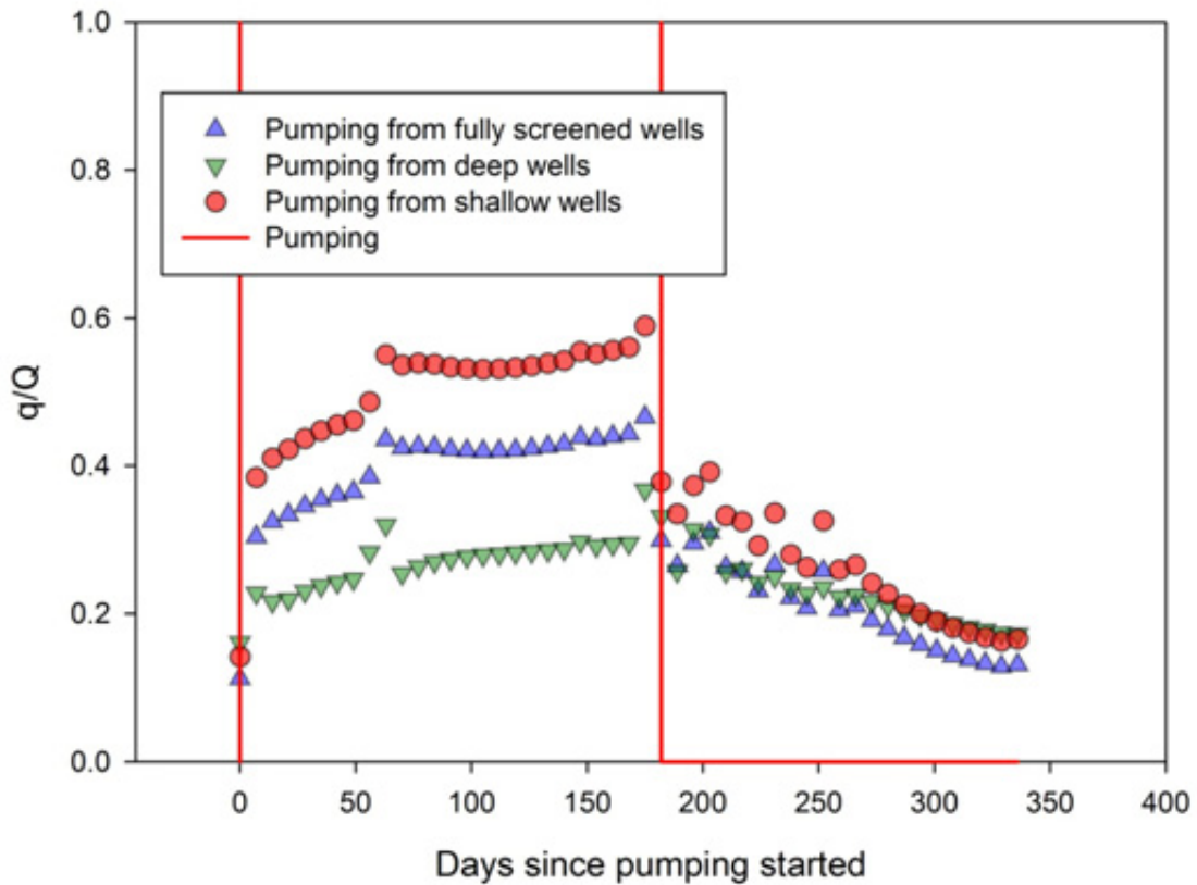
Figure D10: Simulated surface water depletion after 180 days pumping at 4,500 m 3 /day from the deep aquifer >30m, from shallow Holocene sands <20m and from fully screened wells in the Raumati zone expressed as the ratio of depletion rate (q) and pumping rate (Q)
