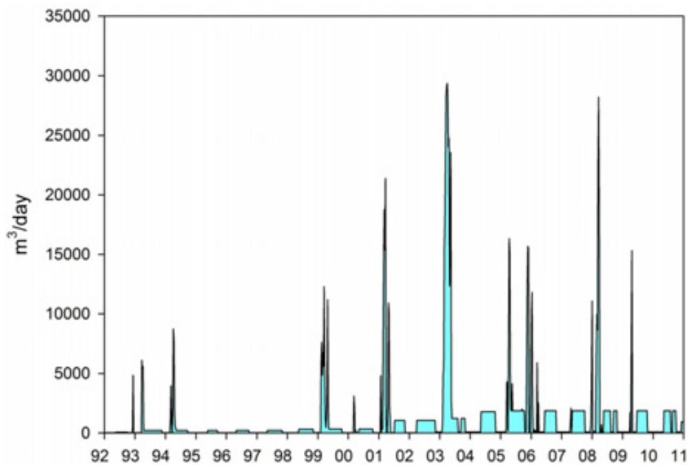
Figure C3: Modelled abstraction in the Waikanae water management zone between 1992 and 2012. The peaks represent the activation of the Waikanae bore field either for water supply or maintenance of the bore field.
