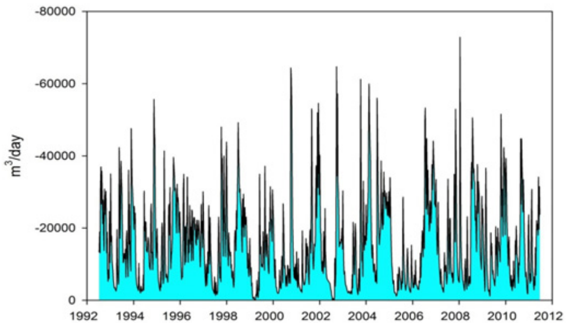
Figure B3: Simulated net natural surface water fluxes to the Mangaone Stream in the Te Horo zone when no groundwater abstraction is occurring. The negative fluxes represent flow from groundwater to the stream (i.e. gaining system). This plot shows the net gain over the entire reach of the Mangaone Stream.
