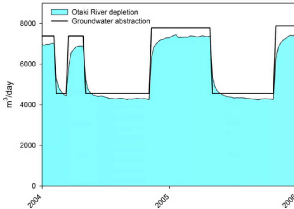
Figure A7: Details of Figure A6-Simulated historic abstraction and associated surface water depletion in the Otaki zone between 2004 and 2006. The plot demonstrates the lag between start and termination of seasonal pumping and surface water depletion. Surface water depletion responds almost immediately to pumping. Abstraction and depletion peak during the summer and continue through the winter at approximately 50% of summer volumes.
