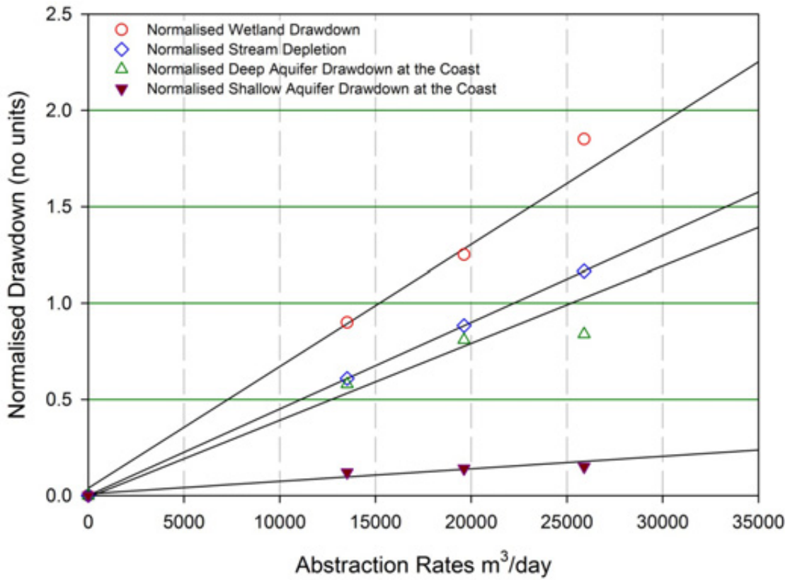
Figure C15: Allocation envelopes abstracting from Q4 and Q6 deep aquifers only. Wetland drawdown is normalised to 0.2m, stream depletion is normalised to 10% of MALF (90L/s) for the entire zone and drawdown at the coast is normalised to 1m. The normalisation values are the maximum allowable depletions or drawdown to limit adverse environmental effects. A normalised wetland drawdown of 1.0 intersects the abstraction rate at 15,000m 3 /day (this abstraction will result in a stream depletion of 0.7 of maximum allowable normalised MALF depletion).
