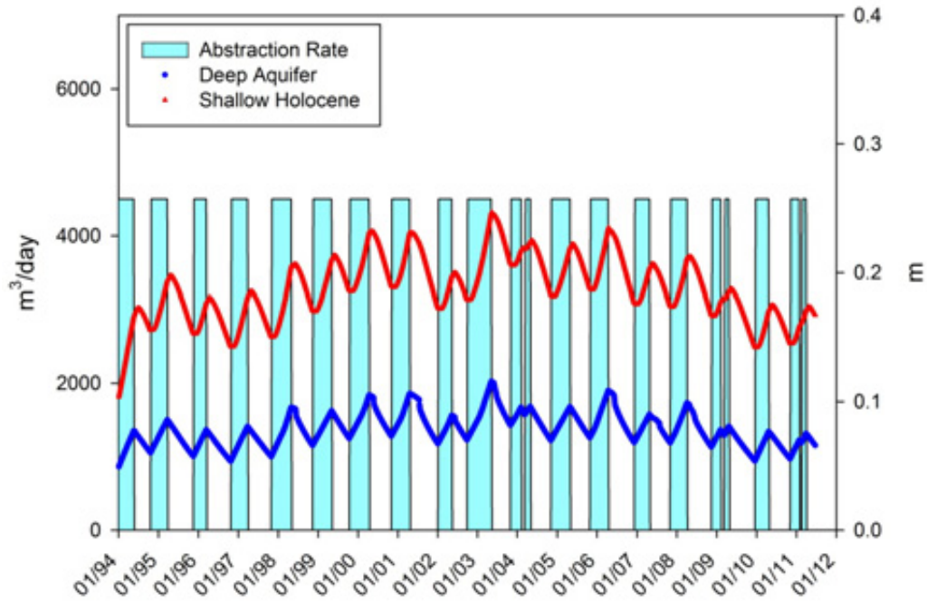
Figure D11: Simulated drawdown resulting from seasonal abstraction at a rate of 4,500 m 3 /day from the shallow Holocene aquifer and deep aquifer respectively between 1994 and 2012
